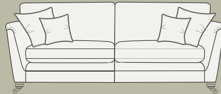
Grand sofa H 950 mm W 2270 mm D 1040 mm
